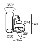
CLUB S 1107 T50 A 284 21 1107 A BA15d / 230-240V / 50-60Hz / TE 1 x QR-LP70 20-50W
