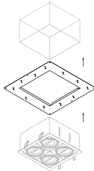
MINIGRID IN 4 PLASTERKIT 202 72 99 04
