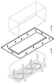
MINIGRID IN 3 PLASTERKIT 202 72 99 03
