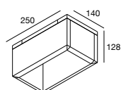
MINIGRID IN ZB 2 50 / QR BOX 202 70 98 02
