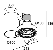
CLUB S HIT-35 A 284 20 1135 E A INCL.1 x CLIP 111 + REFLECTOR FL-35° + GLASS UV-STOP G12 / 230-240V / 50-60Hz / 1 x 1~EVG 1 x HIT 35W
