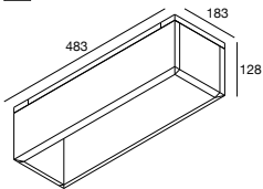
GRID IN ZB 3 QR BOX 202 60 98 03
