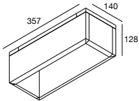
MINIGRID IN ZB 3 50 / QR BOX 202 70 98 03
