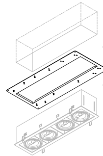
MINIGRID IN 4LINE PLASTERKIT 202 72 99 04L
