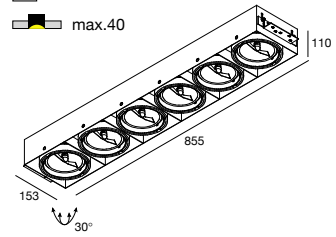
GRID IN TRIMLESS 6LINE QR
